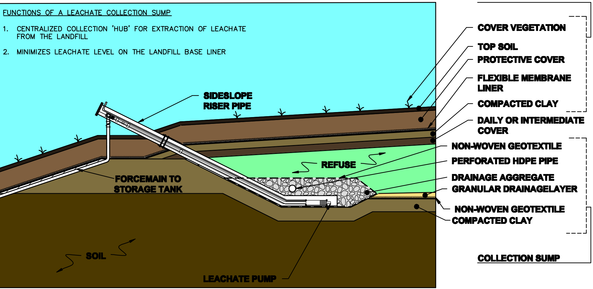
TYPICAL LEACHATE COLLECTION SUMP AND SIDESLOPE RISER PIPE
